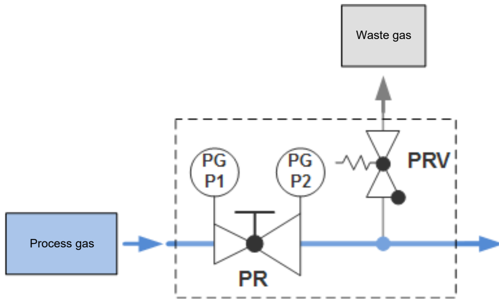
Illustration 2: P&ID U23AC
