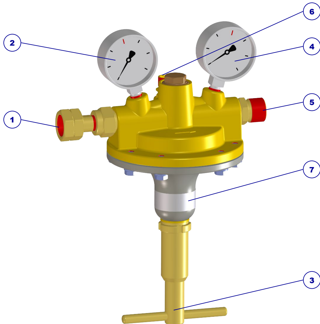
Illustration 1: Pressure regulator design U23AC
