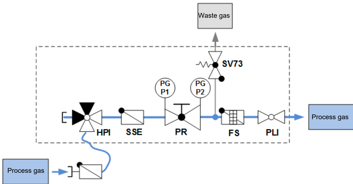
Illustration 2: P&ID MU13AC-SSE
