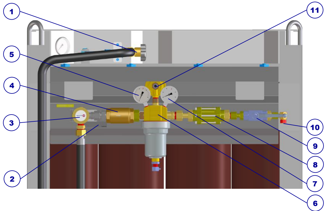
Illustration 1: MU13AC design
