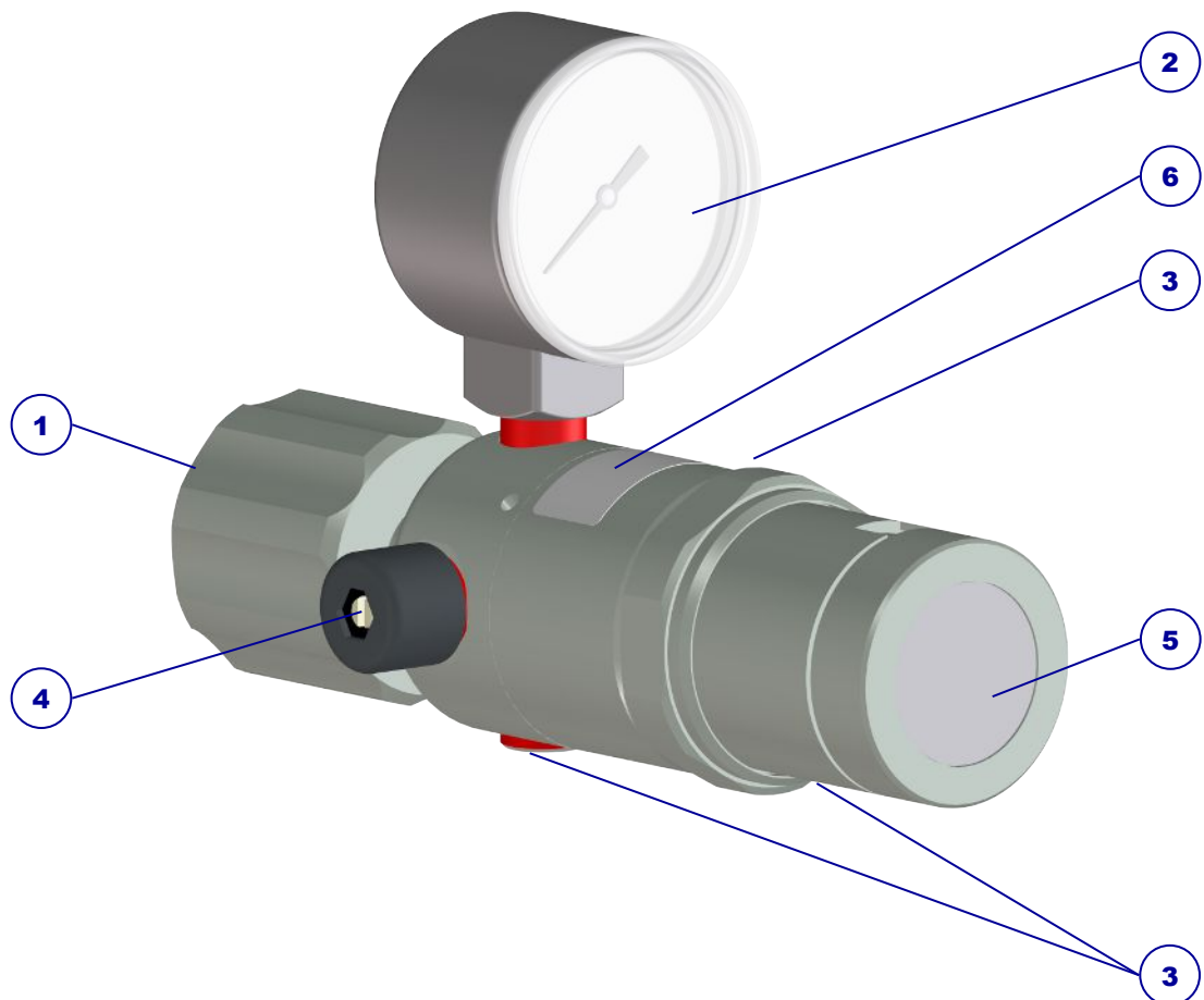
Illustration 1: Pressure regulator design FM35-L
