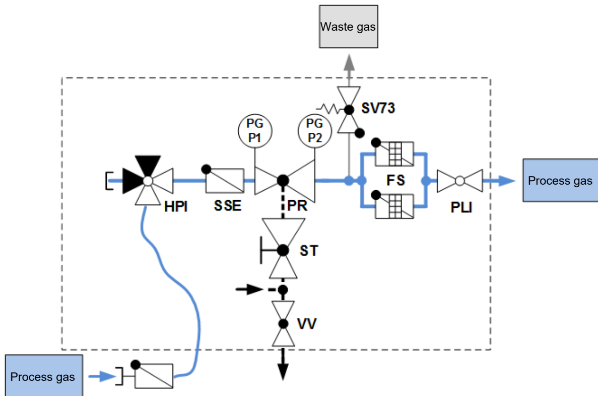
Illustration 2: P&ID BU43F-AC-SSE
