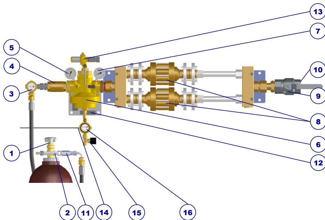
Illustration 1: BU43F-AC-SSE design
