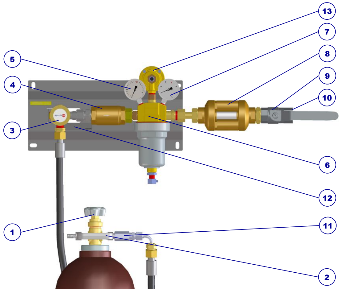
Illustration 1: BU13AC-SSE design
