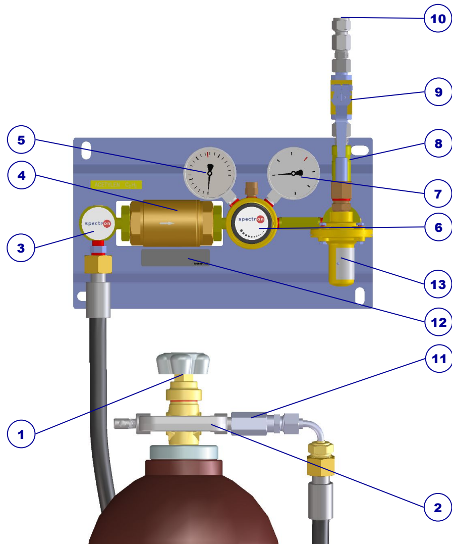
Illustration 1: BT2000AC-SSE design
