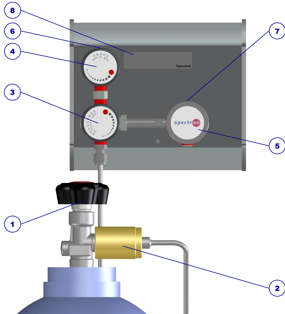
Illustration 1: BM/BE50-1 design
