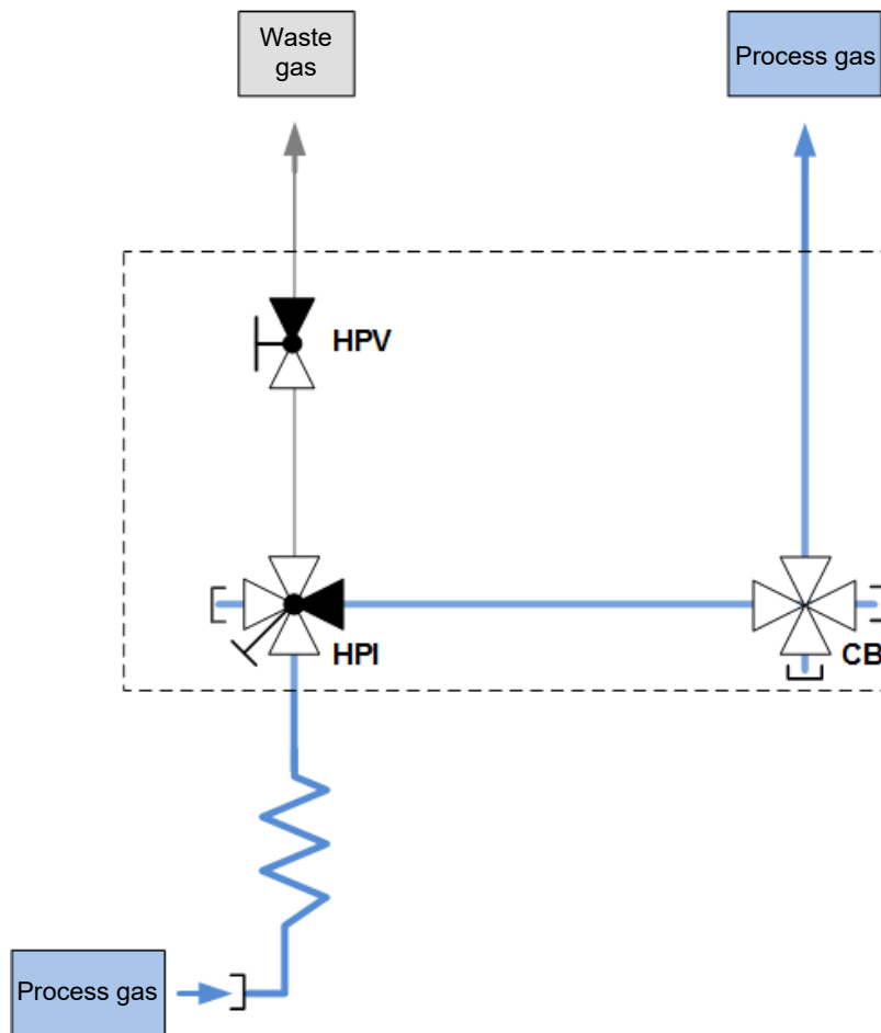
Illustration 2: P&ID BM/BE50-1
