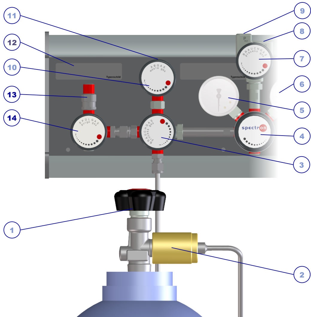
Illustration 1: BE55+56-SP design mounted onto pressure control panel
