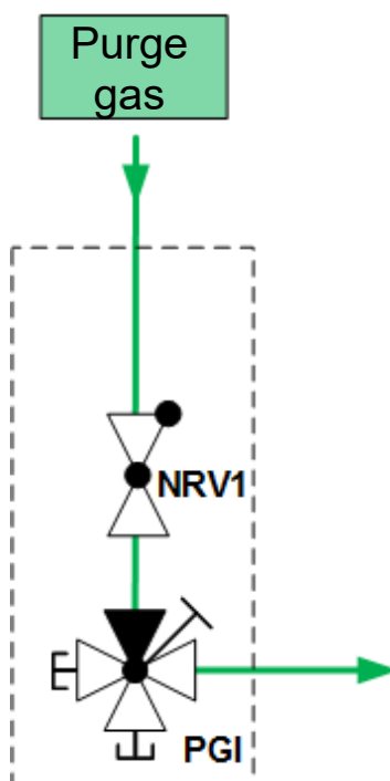
Illustration 2: BE55+56-SP P&ID
