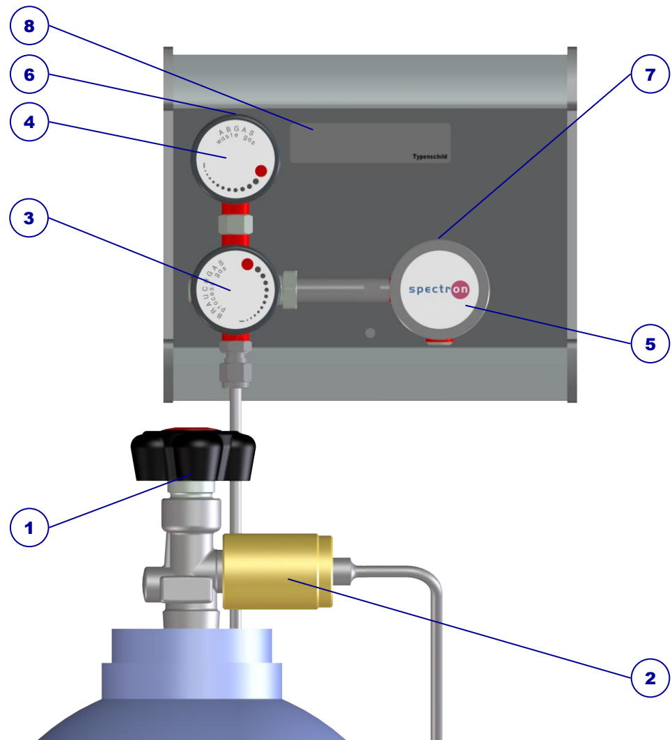
Illustration 1: BM/BE50-1 design
