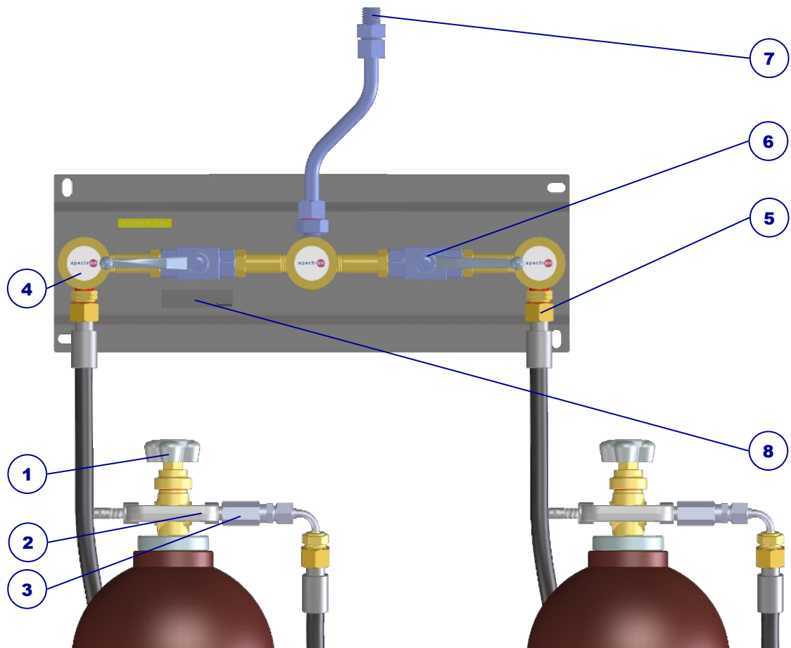
Illustration 1: -2-AC design
