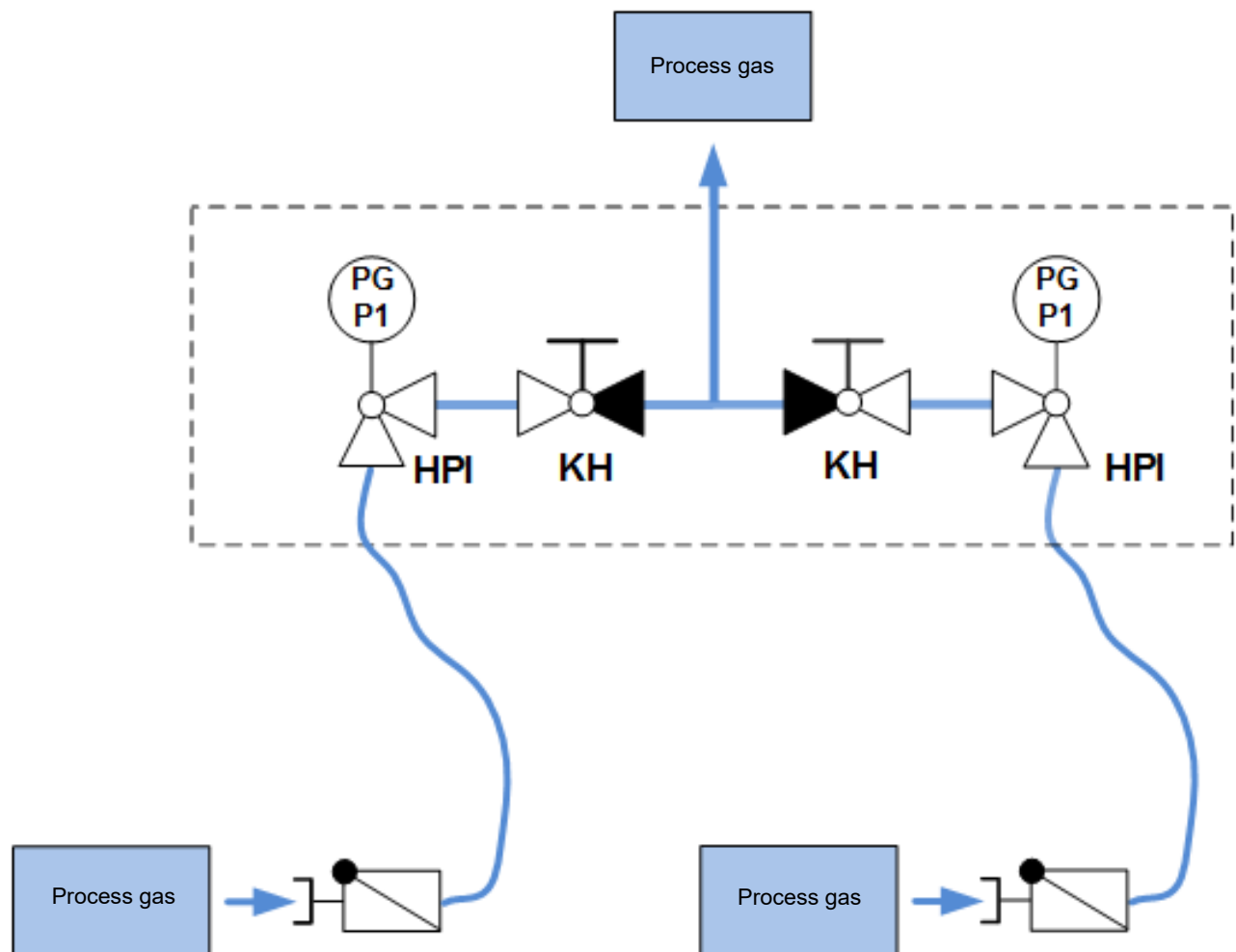
Illustration 2: 2-AC P&ID
