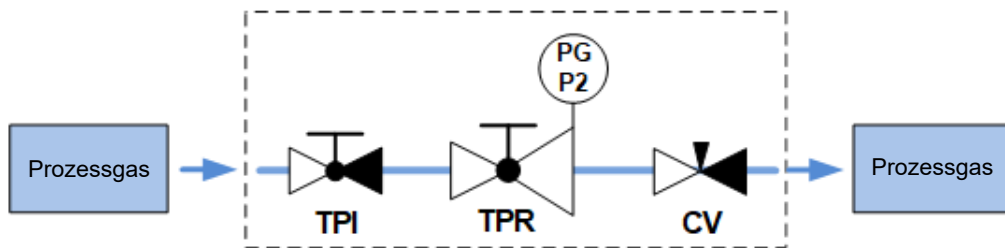
Abb. 2: Schema CRT
