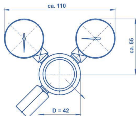
Main dimensions
