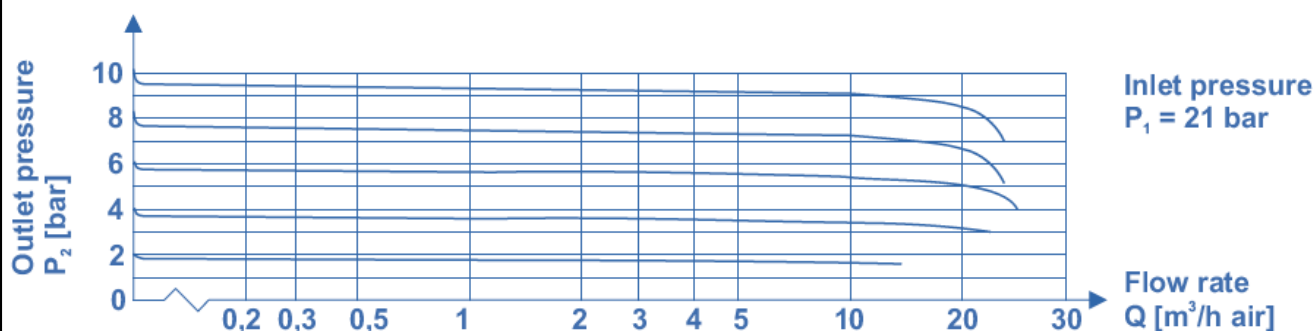
Flow curves BM56-2
