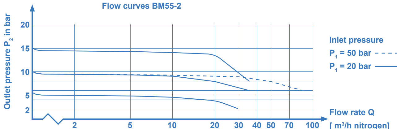
Flow curves BM55-2
